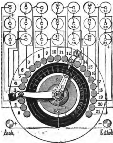
Double collector.
